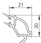
140521 glazing thickness: 20mm
