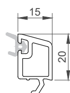
140524 glazing thickness: 24mm
