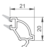
140521 glazing thickness: 20mm
