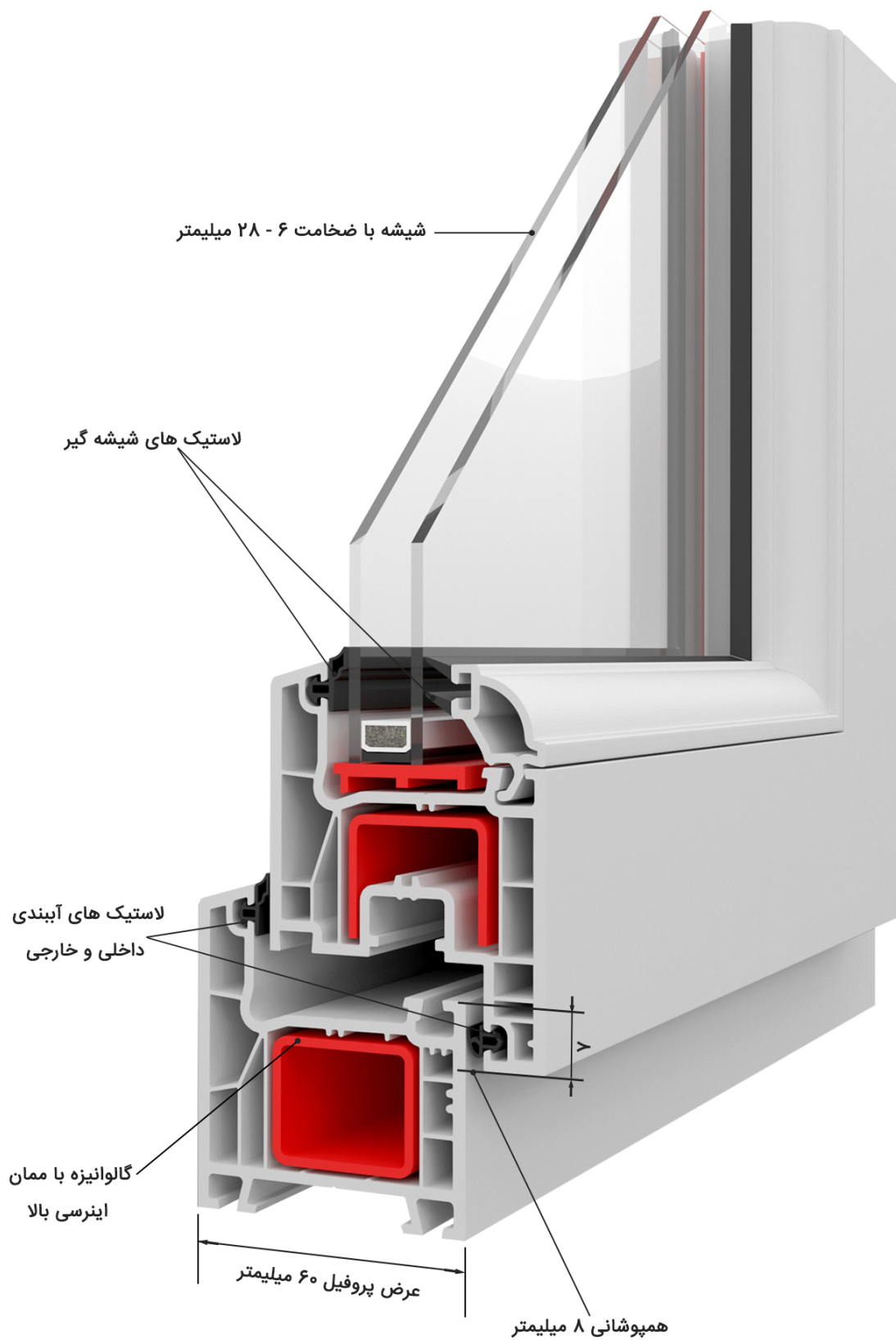
SERIES 6000 4 chamber system / 60mm
