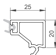
141124 glazing thickness: 24mm
