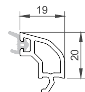
130522 glazing thickness: 22mm
