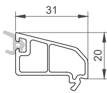
140506 glazing thickness: 6mm
