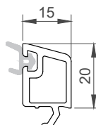
140524 glazing thickness: 24mm
