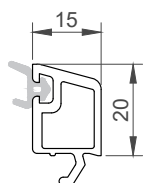
140524 glazing thickness: 24mm
