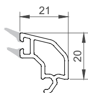
130520 glazing thickness: 20mm
